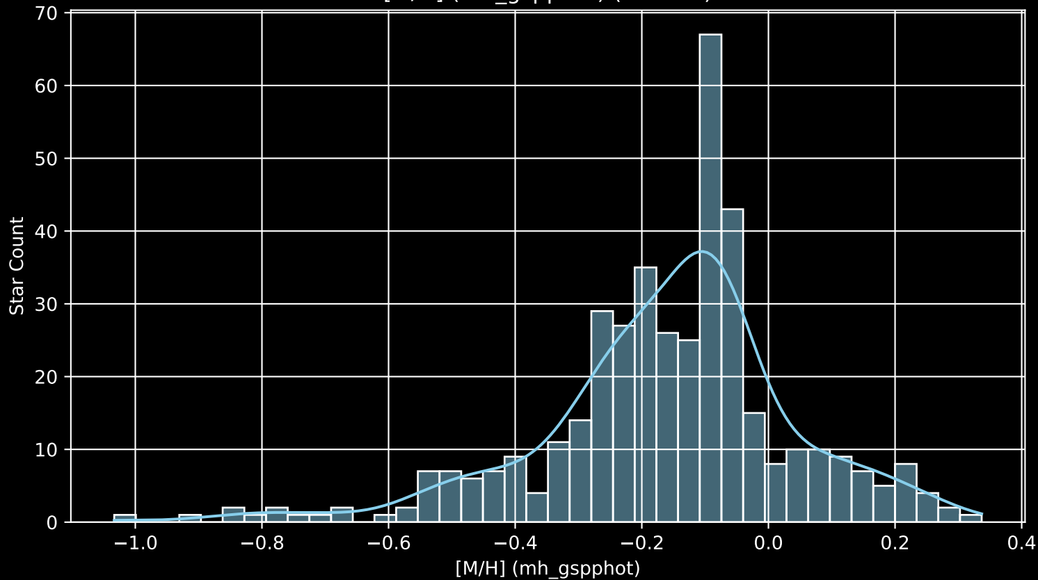
APOGEE DR17 Field: [hip [M/H] (mh_gspphot) (n= 410)
