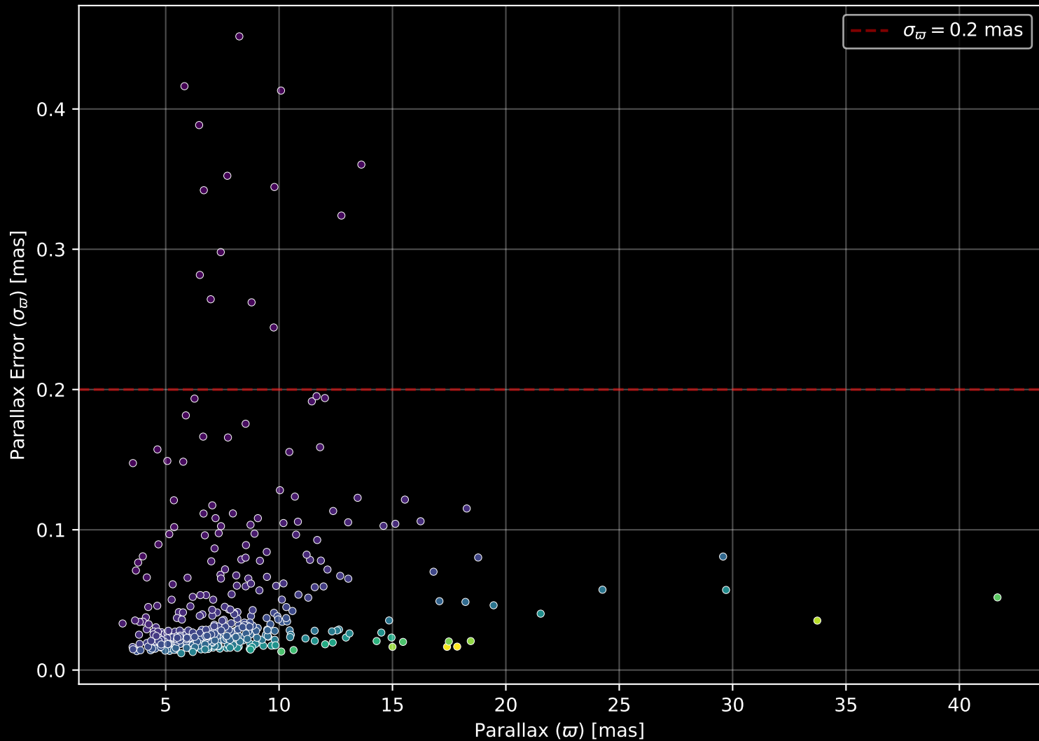
APOGEE DR17 Field: [hip] Parallax Quality (n= 410)
