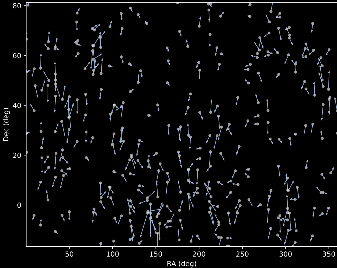
APOGEE DR17 Cluster 1 Proper Motion Vectors (n=318)
