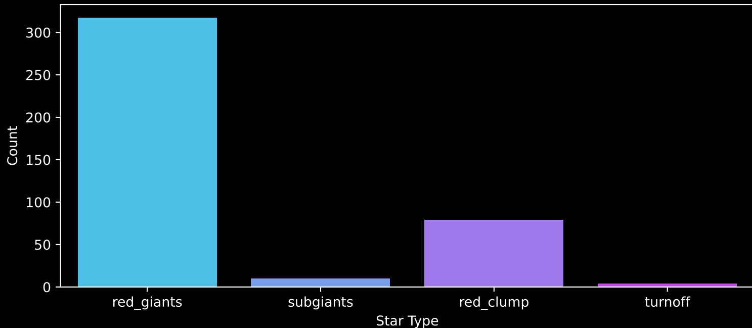
APOGEE DR17 Field: [hip] Count plot of Star Type
