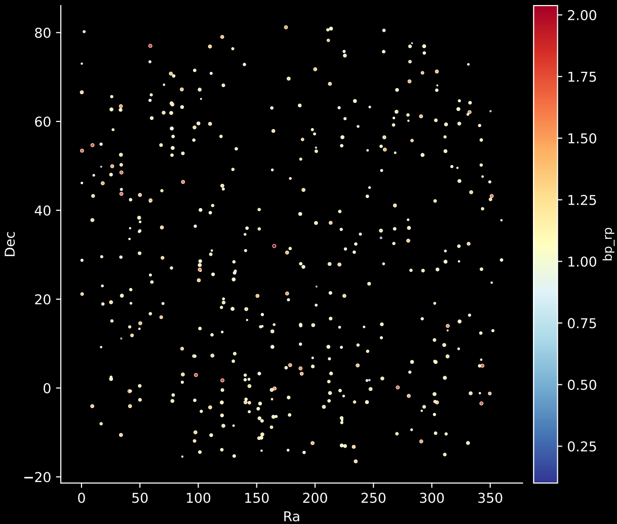
APOGEE DR17 Field: [hip] Stars: 410
