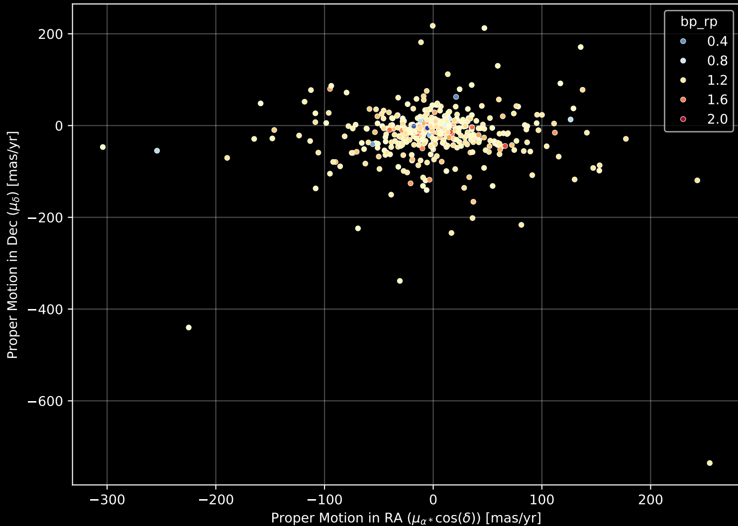
APOGEE DR17 Field: [hip] Proper Motion Diagram (n= 410)
