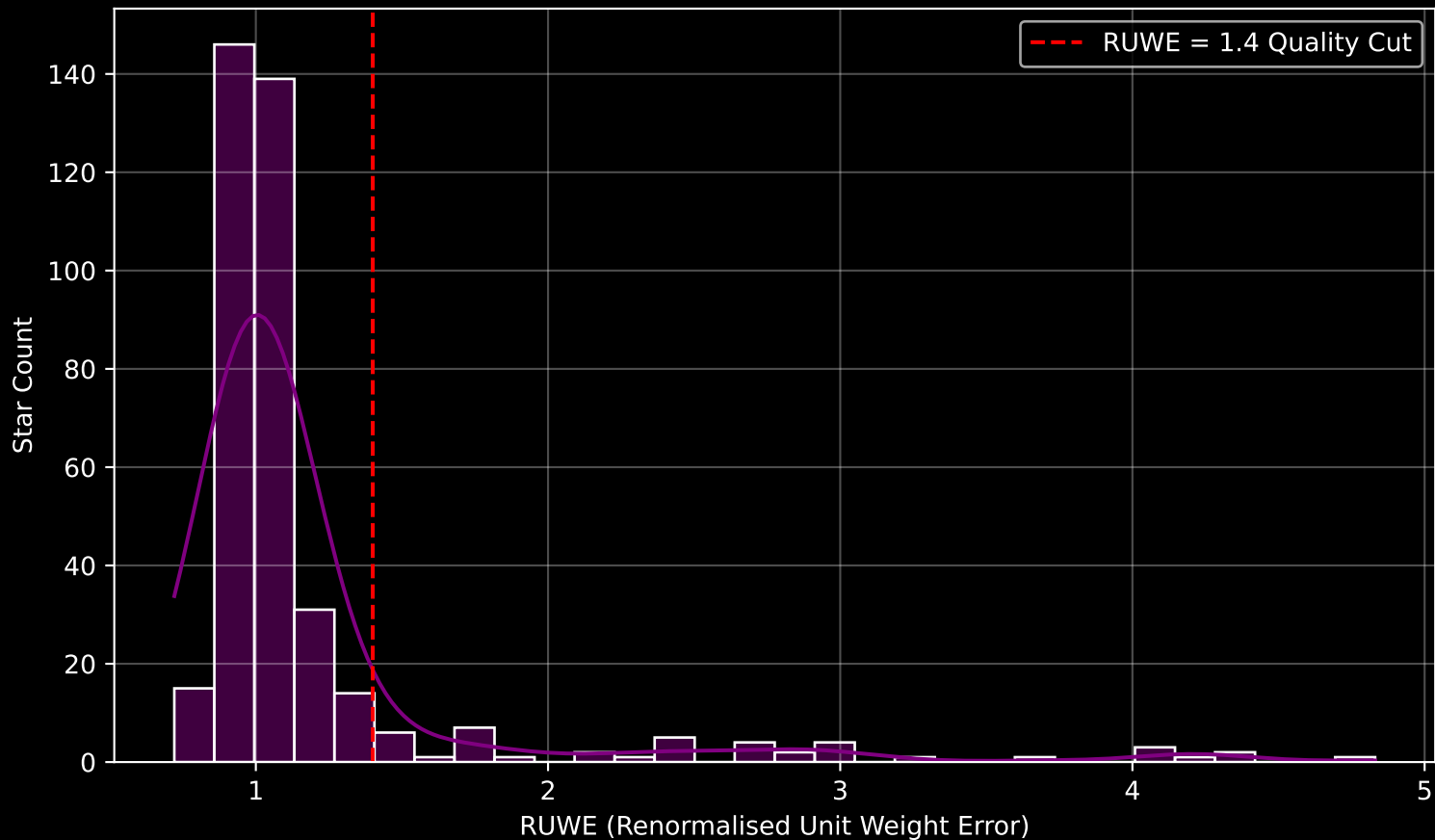
GAPOGEE DR17 Field [hip] RUWE Distribution (n= 387)
